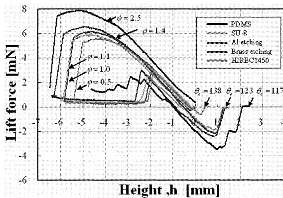
Fig. 11 Experimental Results
