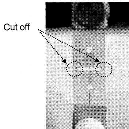
Fig.3 Cut off the side of tab
