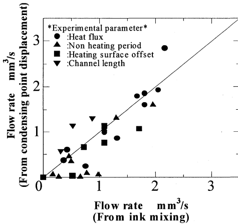
Fig. 2 Flow Rate
