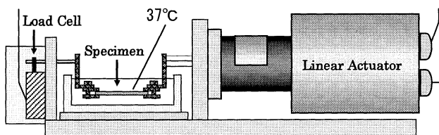
Fig.1 Cyclic culture system for scSAT
