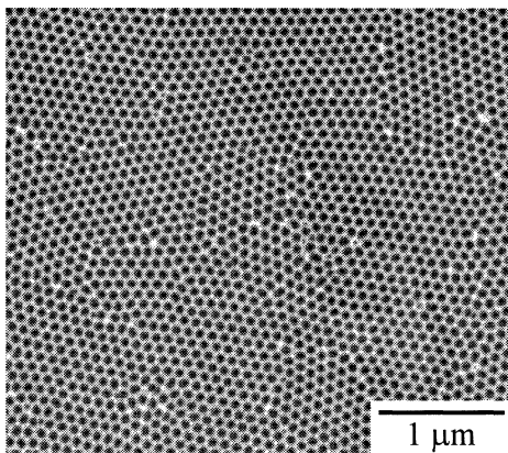
Fig.2 Self-organized anodic porous alumina formed on Al in oxalic acid solution at 40 V for 6 hour.
