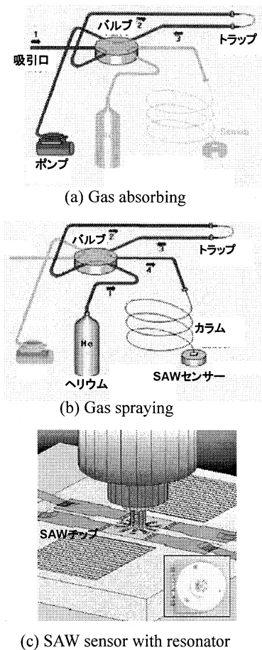
Fig. 3 SAW gas chromatography (EST Corp.)
