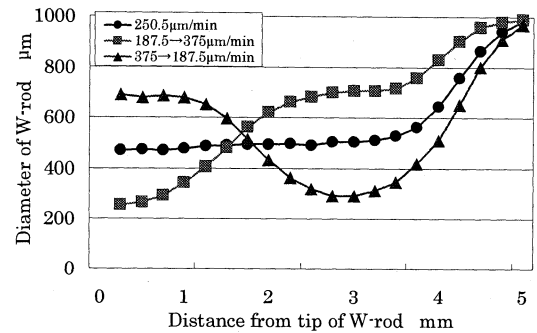
Fig. 4 Machining result for Z-axis controlled
