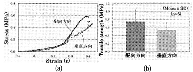
Fig.5 Typical stress-strain curves (a) and tensile strength (b) in longitudinal and vertical directions of Oriented group
