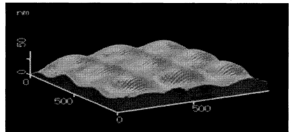
Fig. 2 AFM observation of the periodic micro asperity array on a glass sphere (x-axis and y-axis are 1000 nm in length while the z-axis is 50 nm in length).
