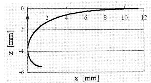
Fig.3 Water surface profile
