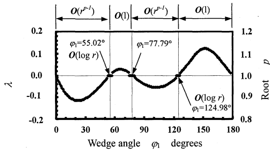
Fig.2 Effect of \phi_1 on stress singularity index \lambda E_2/E_1=0.5, \nu_1=0.27, \nu_2=0.3
