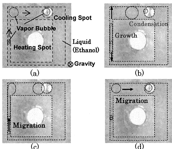
Fig. 1 Vapor Bubbles Behavior
