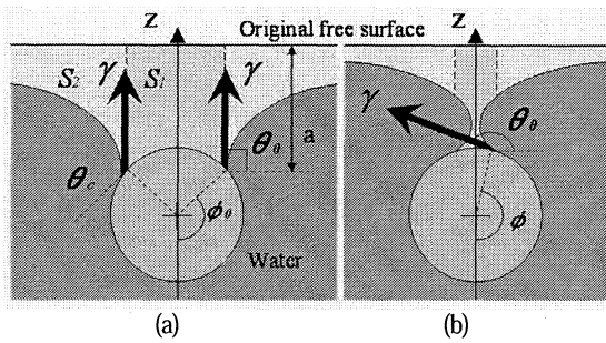
Fig. 4 Maximum surface tension force (a) and maximum depth (b)
