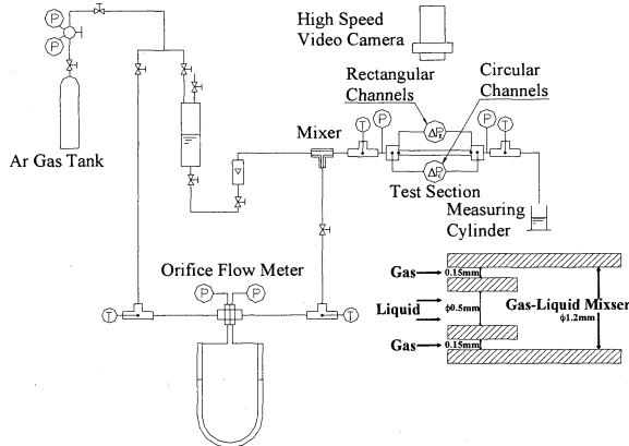
Fig. 1 Experimental apparatus
