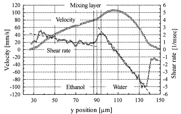
Fig. 2 Axial velocity profile and shear rate
