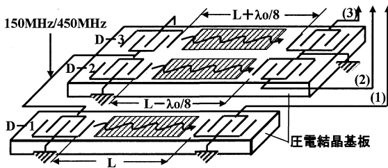
Fig. 6 New SAW gas sensor with three delay lines
