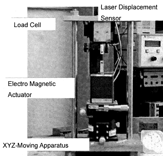
Fig.2 Fatigue tester
