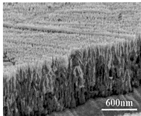
Fig.5 Porous anodic SnO 2 film formed on Sn at 5V in sodium hydroxide.
