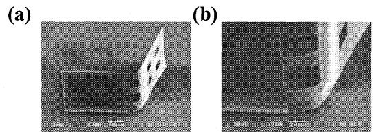
Fig.5 Self-assembled hinge
