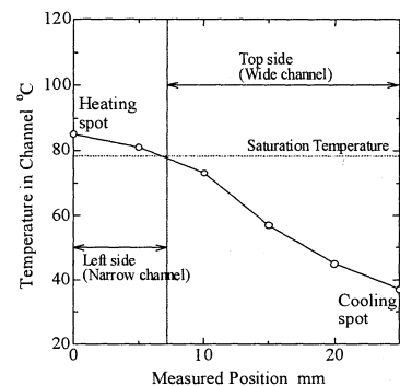
Fig. 3 Liquid Temperature Distribution
