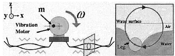
Fig. 13 Rotational vibration of the supporting legs
