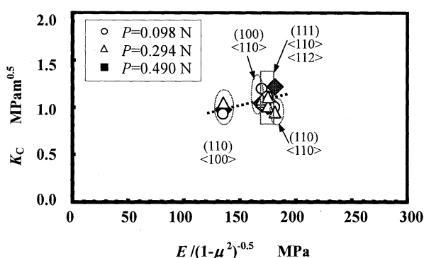
Fig. 5 Relationship between Fracture toughness and E/(1-\mu^2)^{0.5}
