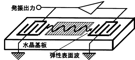
Fig. 4 SAW oscillator-type gas sensor
