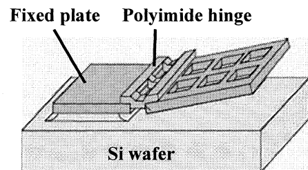
Fig. 2 Hinged mechanism
