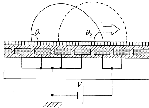
Fig. 6 Continuous motion of ungrounded droplet
