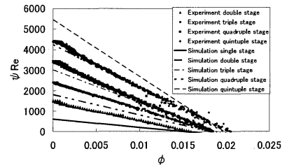
Fig. 4 Pressure characteristics for multiple rotors.
