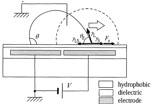
Fig. 2 Principle of EWOD. The droplet is grounded.
