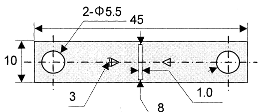
Fig.1 Dimension of Polypropylene tab
