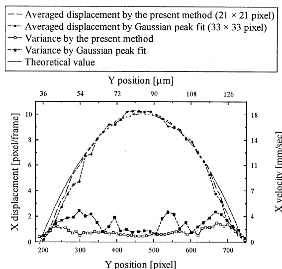
Fig. 4 Time-averaged axial velocity profiles in microtube (7)
