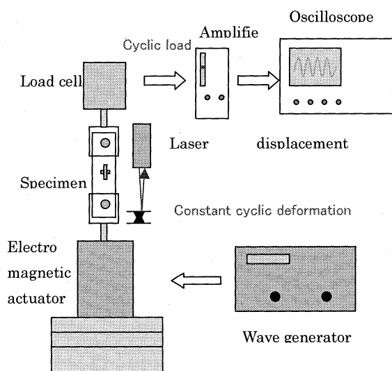
Fig. 3 Block diagram of fatigue testing system.
