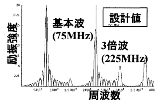
Fig. 8 Design results for new transducer
