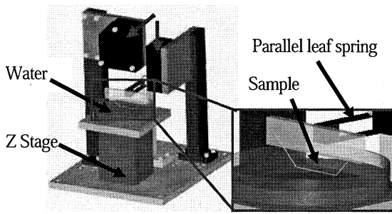
Fig. 9 Experimental setup
