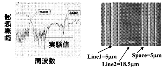
(a) Frequency characteristics (b) Electrodes
