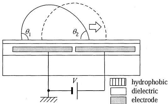
Fig. 4 ungrounded droplet
