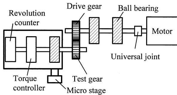
Fig.5 Fatigue testing apparatus for spur gear.
