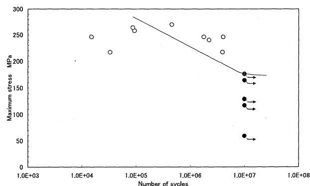
Fig.6 S-N curves of Al bonding wire
