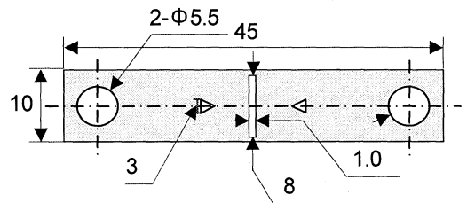
Fig.2 Dimension of Polypropylene tab
