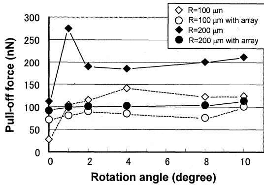
Fig. 3 Pull-off force as a function of misalignment angle of the array pattern of the silicone plane with respect to the glass sphere with and without array pattern of 100 and 200 \mu\text{m} in curvature measured in about 25%Rh.
