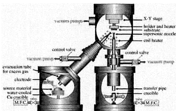
Fig. 4 Schematic diagram of SFJ-PVD apparatus.
