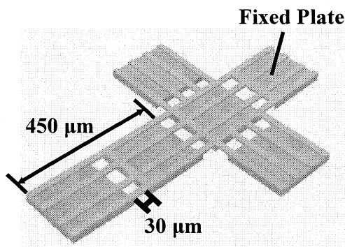
Fig.7 Planar structure for assembling a microcube.
