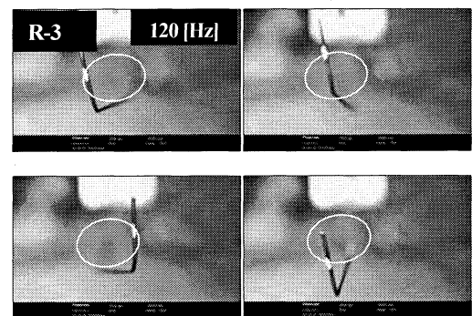
Fig. 14 Vibration of the supporting leg in air
