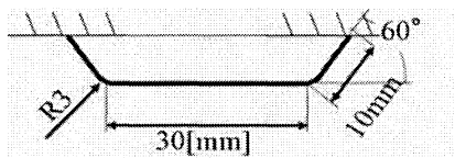
Fig. 10 Specimen's geometry
