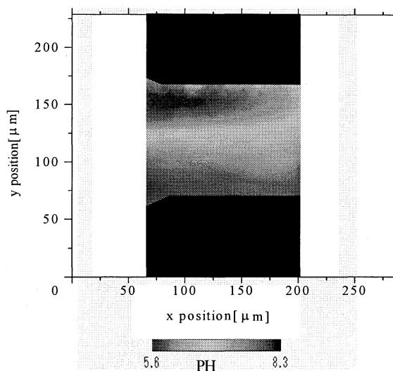
Fig. 5 pH distribution obtained by Micro LIF (19)
