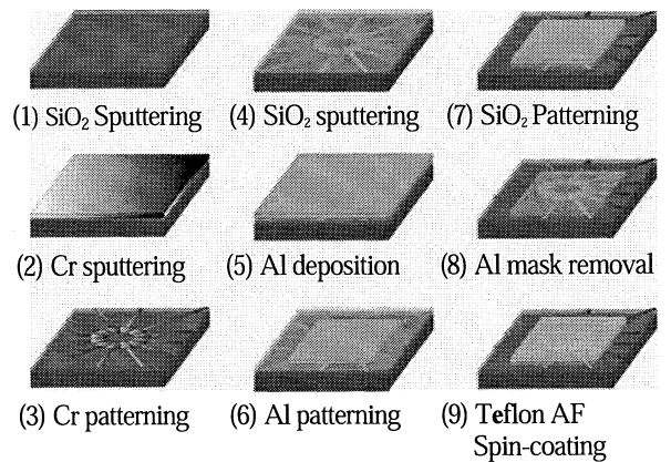
Fig. 11 Fabrication process for stator
