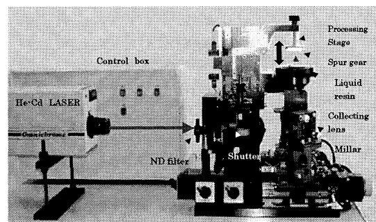
Fig.2 Stereo lithography system apparatus with Helium-Cadmium laser.
