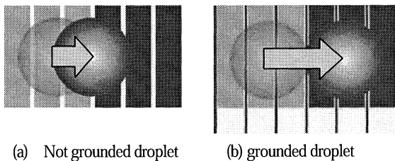
Fig. 10 Motion of the droplet
