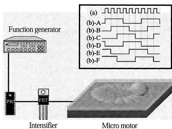
Fig. 12 Experimental setup for droplet transration
