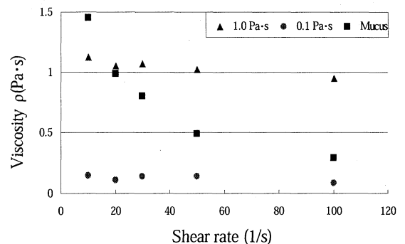
Fig.7 Relationship between shear rate and viscosity for mucus liquid as compared with viscosity standard solution
