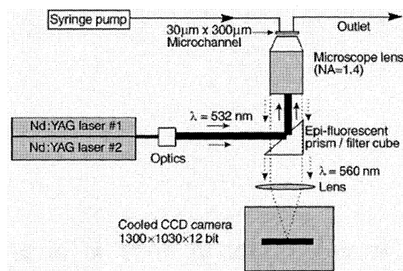
Fig. 1 Micro PIV system (3)
