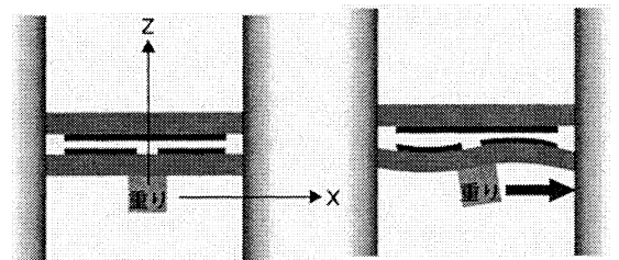
(a) Without acceleration (b) With acceleration Fig. 1 Acceleration sensor
