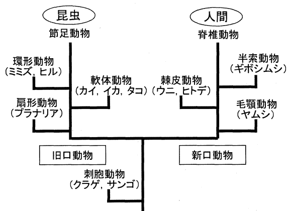
Fig. 4 Genealogical tree
