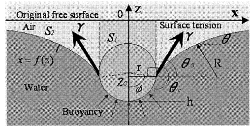
Fig.2 2D-model of a supporting leg.
