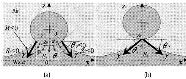
Fig. 5 Pull-off force
