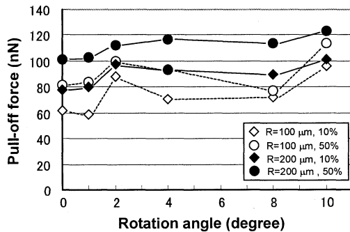
Fig. 4 Pull-off force as a function of misalignment angle of the array pattern of the silicone plane with respect to the glass sphere with array pattern of 100 and 200 \mu\text{m} in curvature measured in about 10 and 50%Rh.
