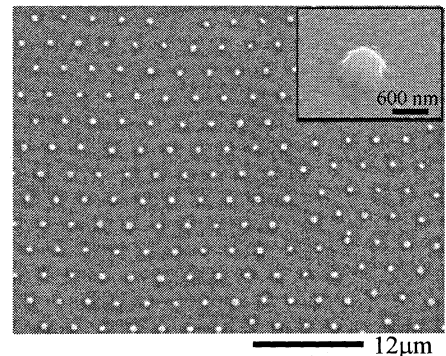
Fig. 3 SEM image of surface of anodized silicon at current density of 25 \text{ mAcm}^{-2} for 2 min in a HF-containing solution.
