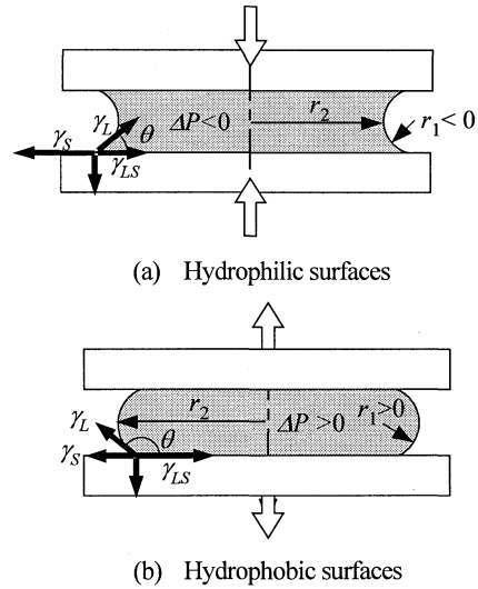
Fig. 2 Meniscus force between two planar surfaces
