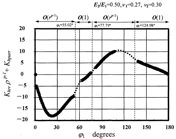
Fig.3 Effect of wedge angle on intensity of singularity field ( K_{hrr} \rho^{p-1} + K_{hpar} ), \rho=0.00001
